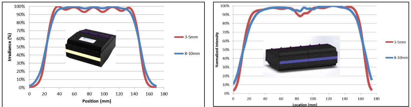
Figure 4: Uniformity of Irradiance
