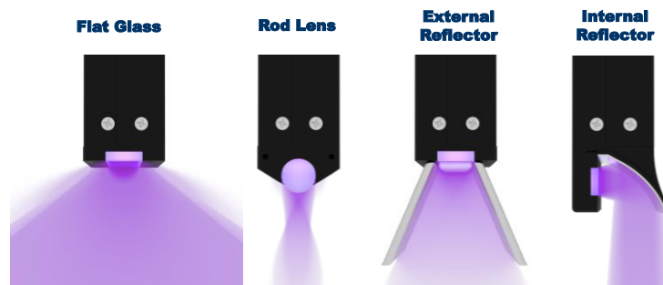
Figure 5: Illustration of How Optics Impact Concentration or Spread of UV LED Light
