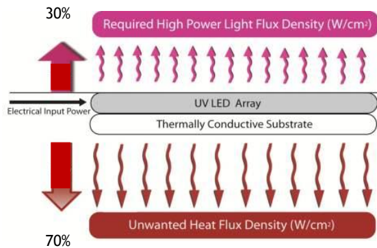
Figure 6: Conversion of Electrical Input Power into UV LED Output and Dissipated Heat
