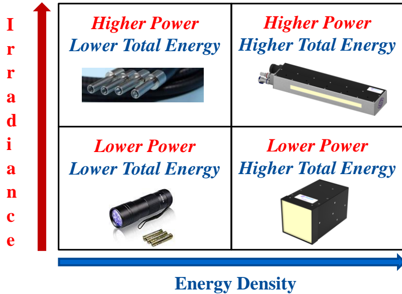
Figure 2: Irradiance vs Energy Density can be De-coupled in UV LED Source Design.
